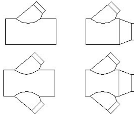
Fittings with 45° Conical Taps
