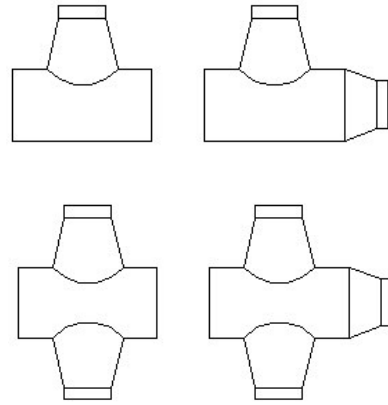
Fittings with 90° Conical Taps
