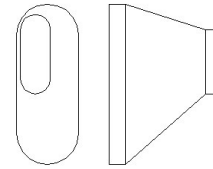
Oval to Oval Non-Concentric Transition
