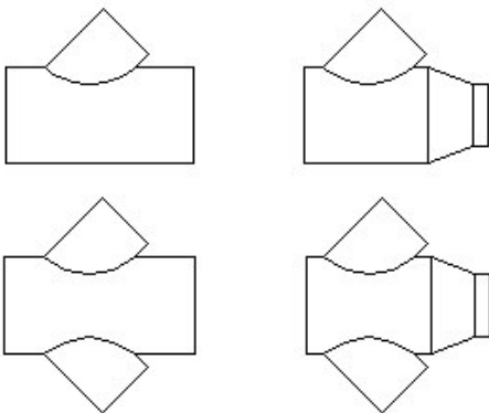
Fittings with 45° Straight Taps
